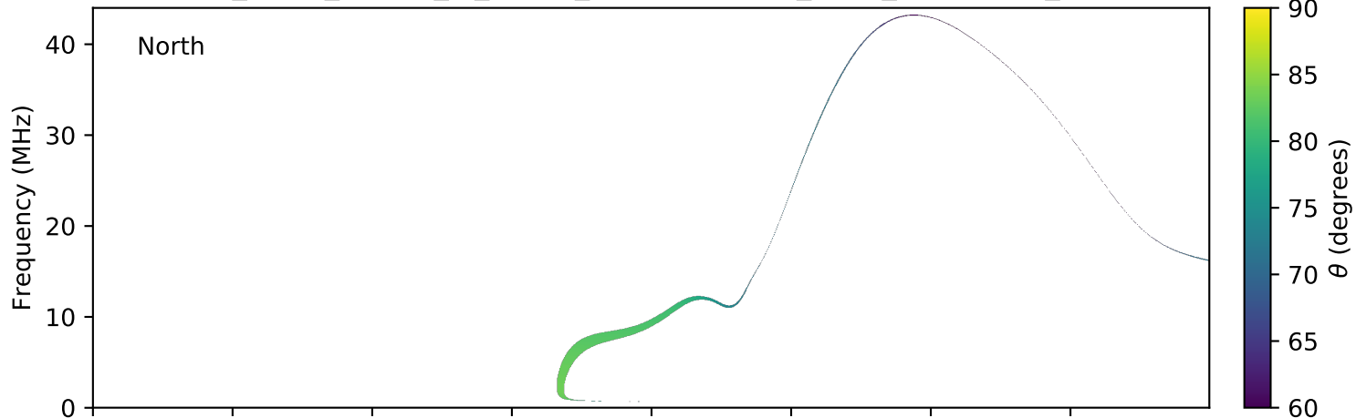
expres_earth_jupiter_io_jrm09_lossc-wid1deg_3kev_20060401_v01.cdf
