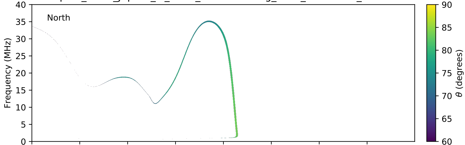
expres_earth_jupiter_io_isaac_lossc-wid1deg_3kev_20060430_v01.cdf
