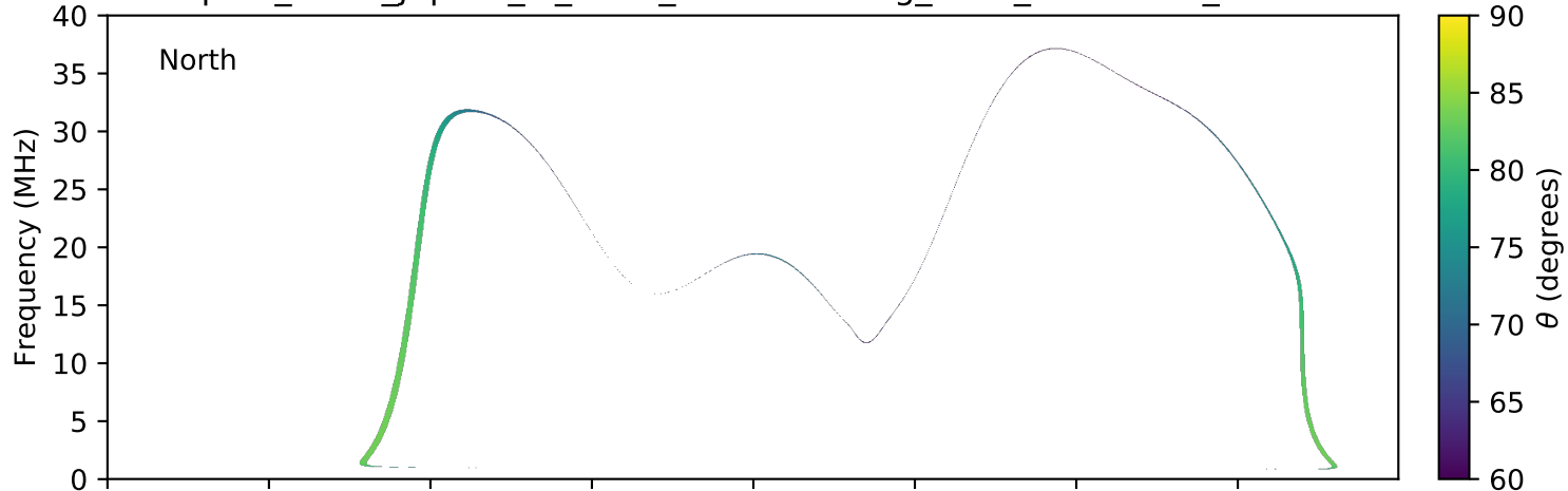
expres_earth_jupiter_io_isaac_lossc-wid1deg_3kev_20060426_v01.cdf
