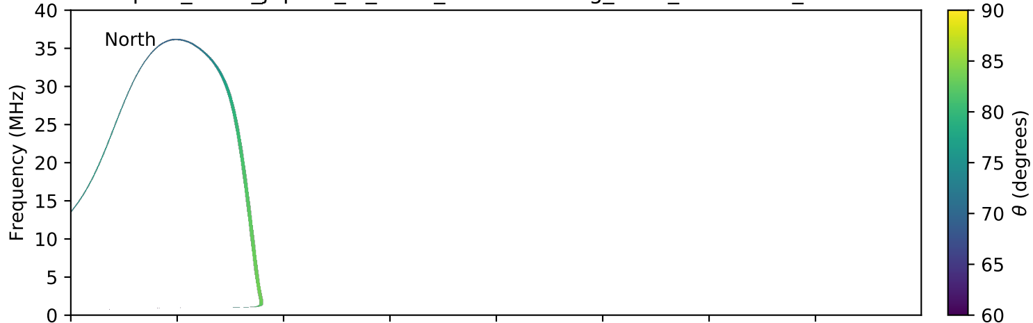
expres_earth_jupiter_io_isaac_lossc-wid1deg_3kev_20060425_v01.cdf
