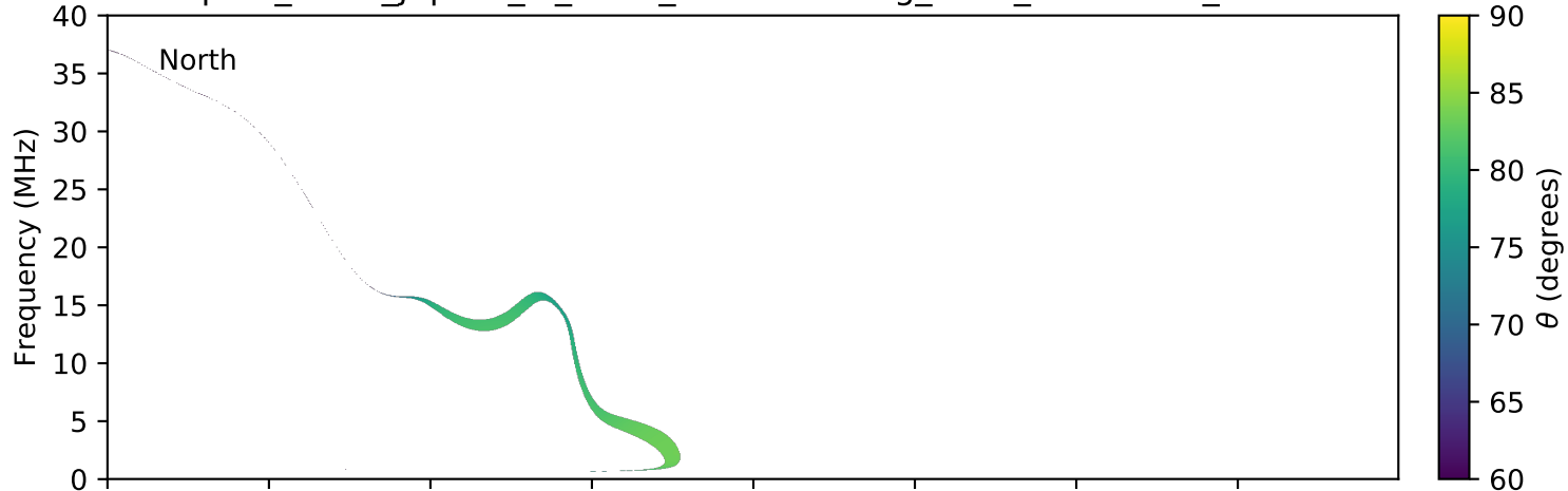
expres_earth_jupiter_io_isaac_lossc-wid1deg_3kev_20060423_v01.cdf
