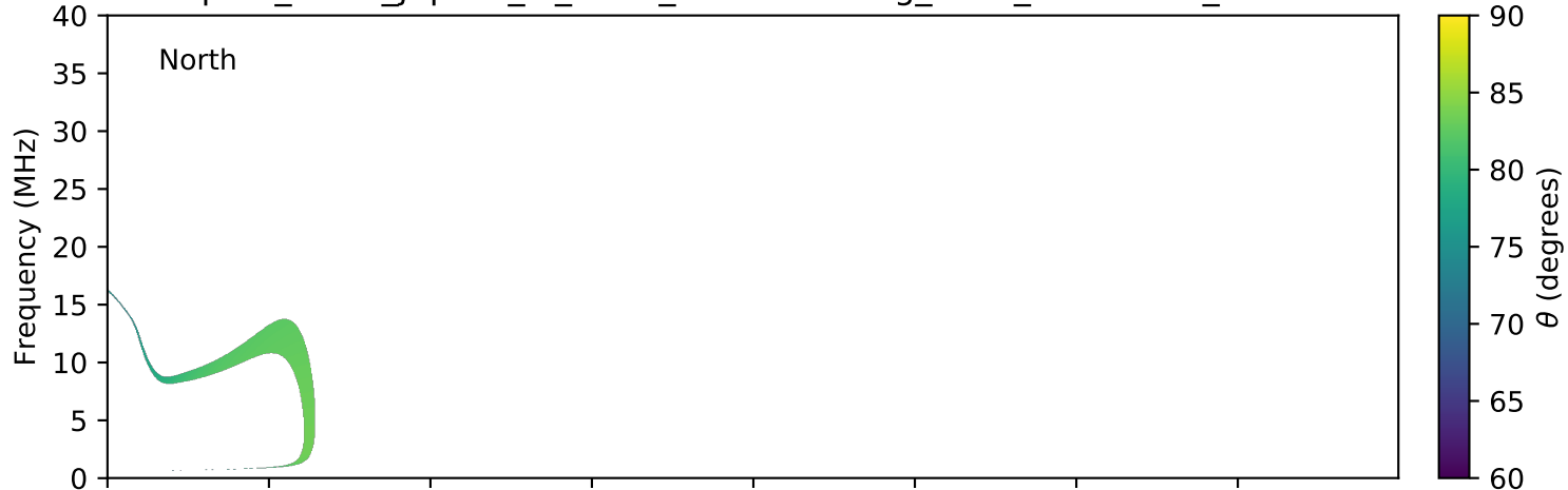
expres_earth_jupiter_io_isaac_lossc-wid1deg_3kev_20060418_v01.cdf
