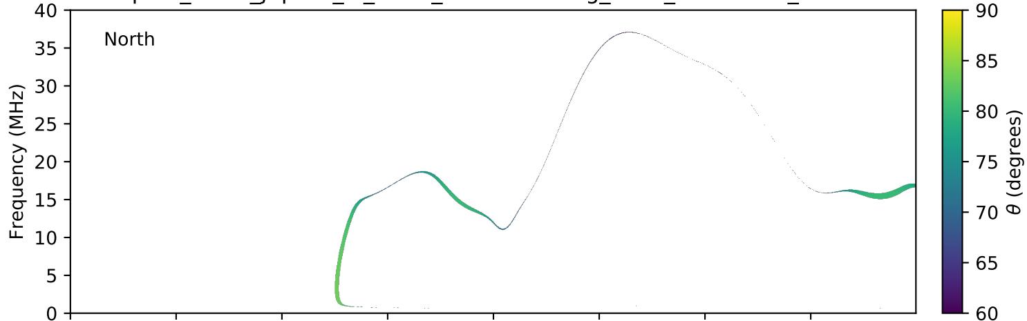
expres_earth_jupiter_io_isaac_lossc-wid1deg_3kev_20060417_v01.cdf
