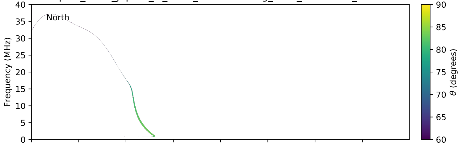
expres_earth_jupiter_io_isaac_lossc-wid1deg_3kev_20060416_v01.cdf
