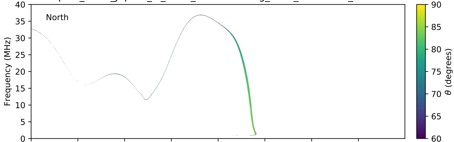
expres_earth_jupiter_io_isaac_lossc-wid1deg_3kev_20060414_v01.cdf
