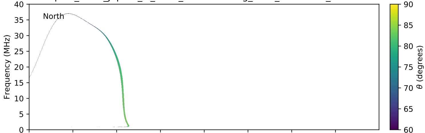
expres_earth_jupiter_io_isaac_lossc-wid1deg_3kev_20060409_v01.cdf
