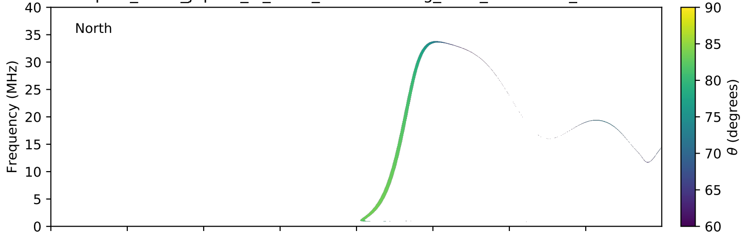
expres_earth_jupiter_io_isaac_lossc-wid1deg_3kev_20060408_v01.cdf
