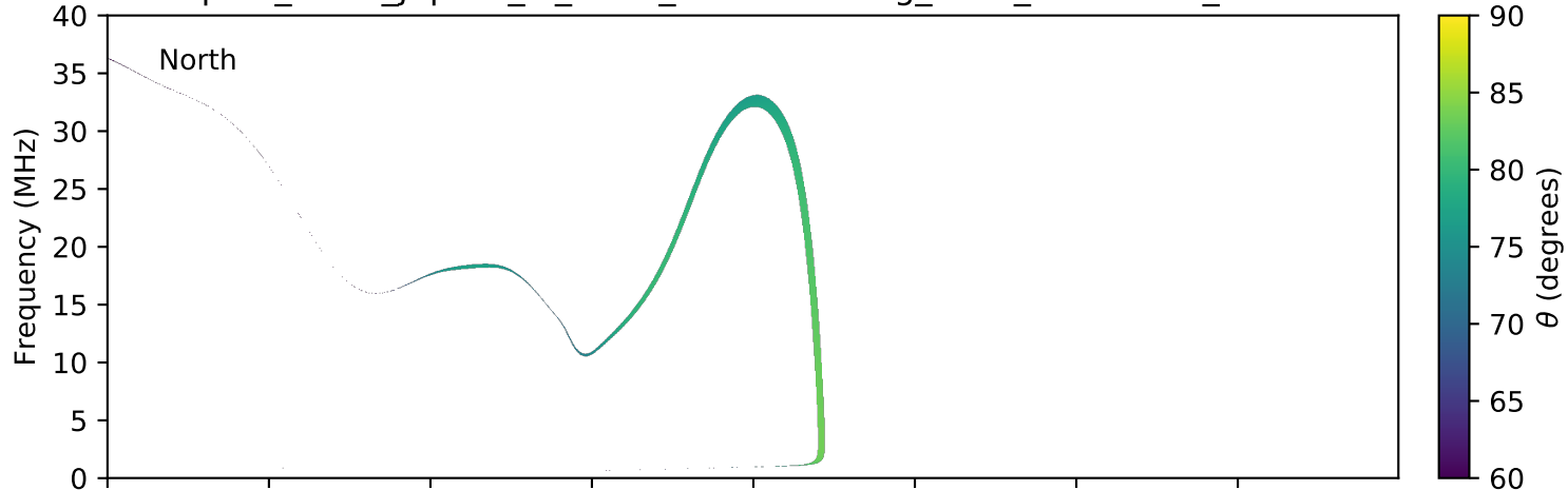
expres_earth_jupiter_io_isaac_lossc-wid1deg_3kev_20060407_v01.cdf
