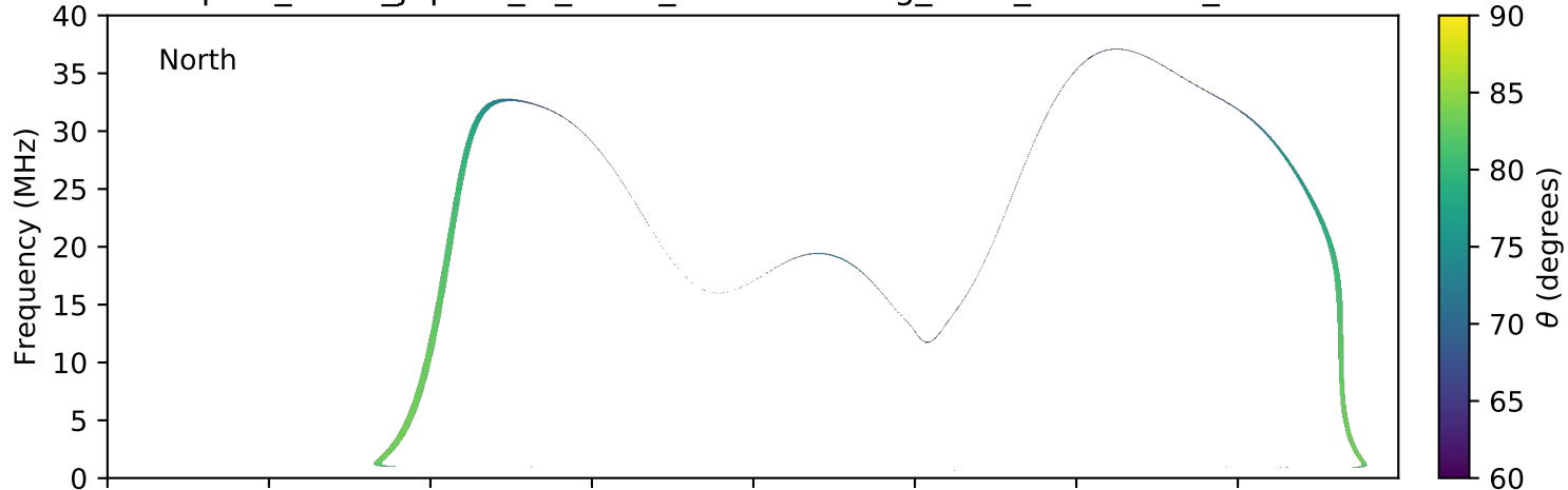
expres_earth_jupiter_io_isaac_lossc-wid1deg_3kev_20060403_v01.cdf
