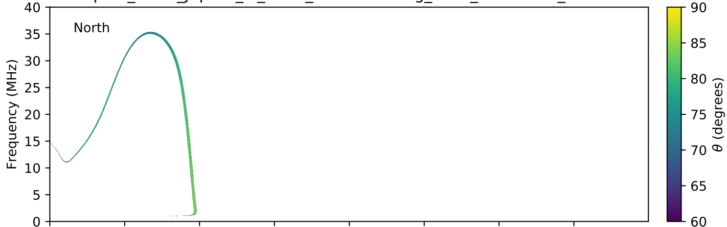
expres_earth_jupiter_io_isaac_lossc-wid1deg_3kev_20060402_v01.cdf
