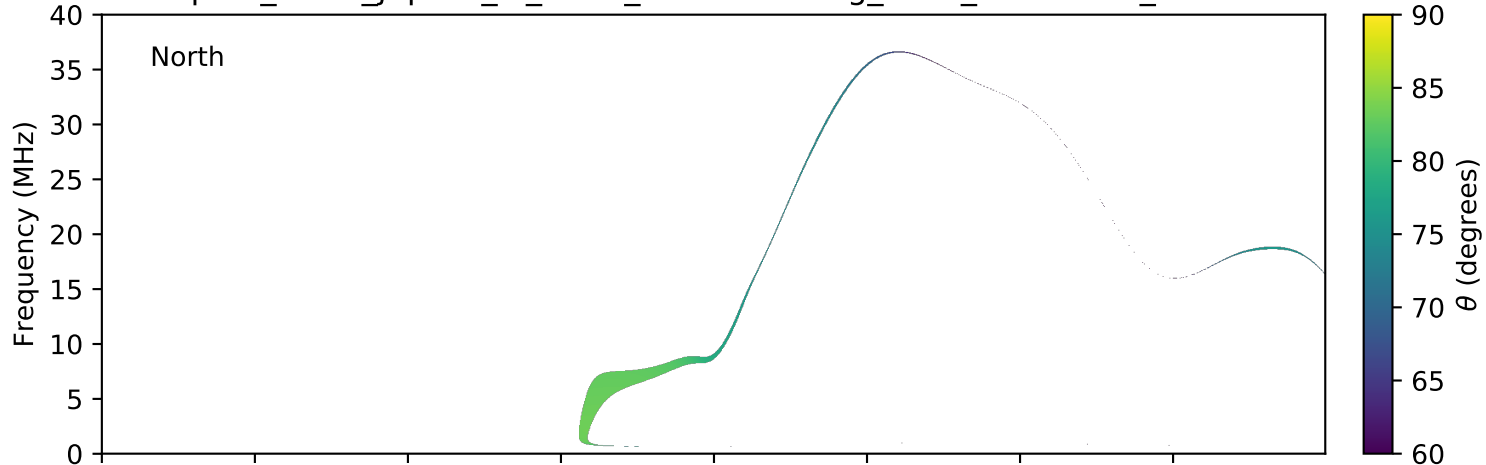
expres_earth_jupiter_io_isaac_lossc-wid1deg_3kev_20060401_v01.cdf
