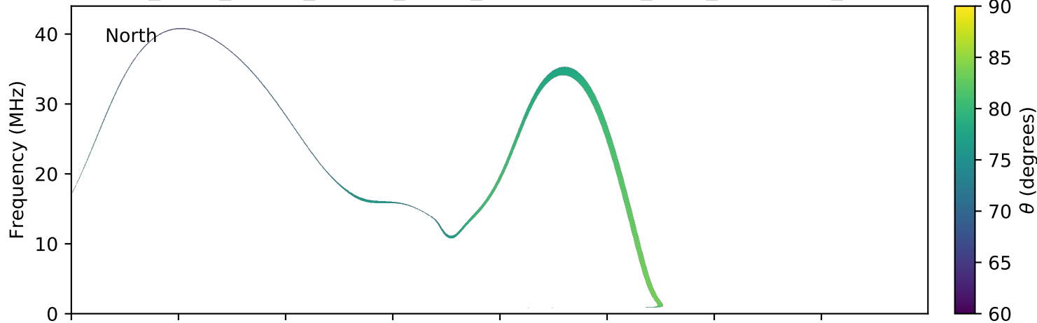
expres_earth_jupiter_europa_jrm09_lossc-wid1deg_3kev_20060412_v01.cdf
