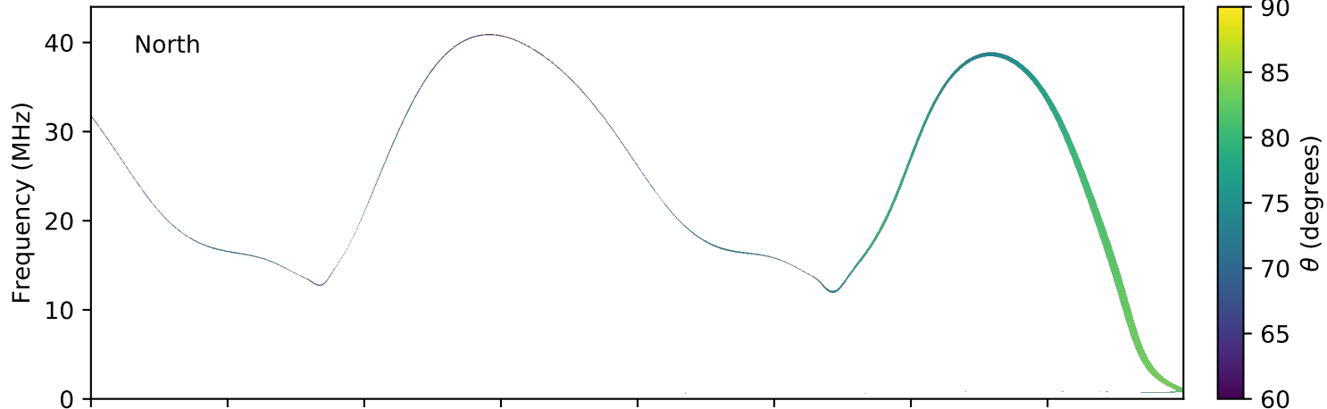
expres_earth_jupiter_europa_jrm09_lossc-wid1deg_3kev_20060401_v01.cdf
