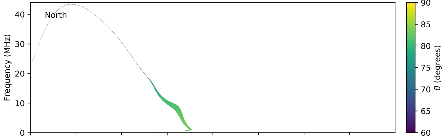
expres_earth_jupiter_io_jrm09_lossc-wid1deg_3kev_20060331_v01.cdf
