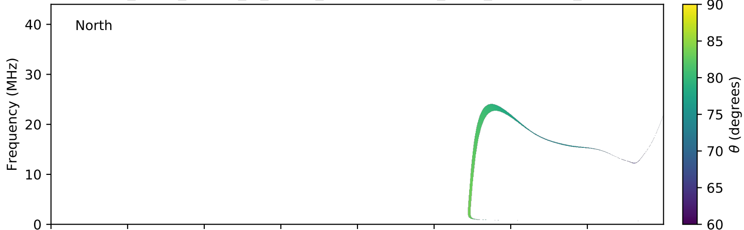
expres_earth_jupiter_io_jrm09_lossc-wid1deg_3kev_20060330_v01.cdf
