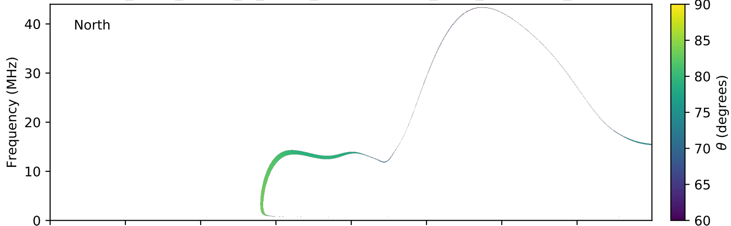
expres_earth_jupiter_io_jrm09_lossc-wid1deg_3kev_20060325_v01.cdf
