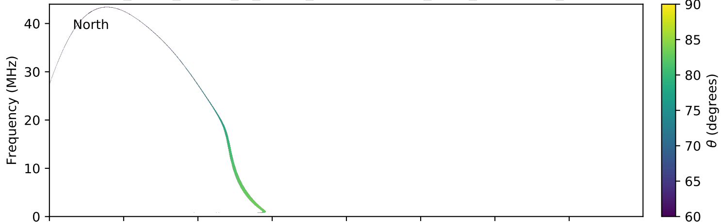
expres_earth_jupiter_io_jrm09_lossc-wid1deg_3kev_20060324_v01.cdf
