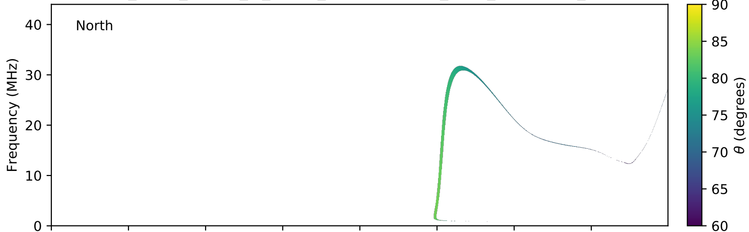
expres_earth_jupiter_io_jrm09_lossc-wid1deg_3kev_20060323_v01.cdf
