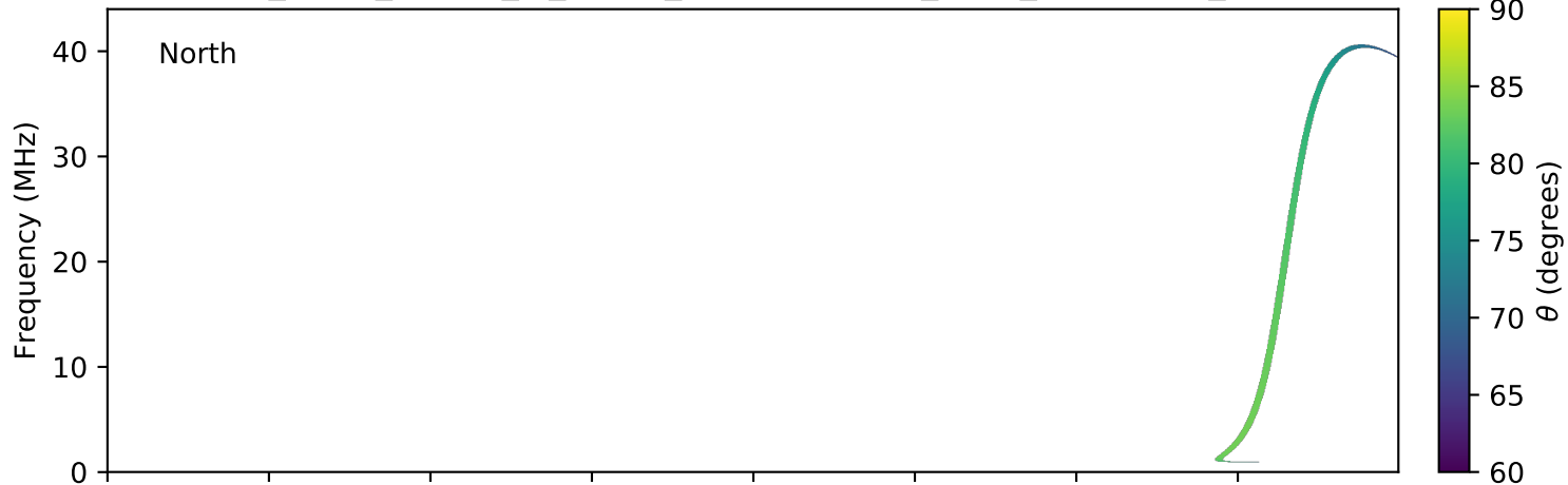
expres_earth_jupiter_io_jrm09_lossc-wid1deg_3kev_20060321_v01.cdf
