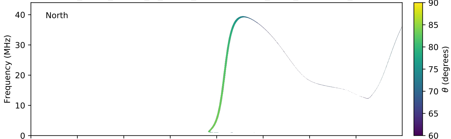
expres_earth_jupiter_io_jrm09_lossc-wid1deg_3kev_20060309_v01.cdf
