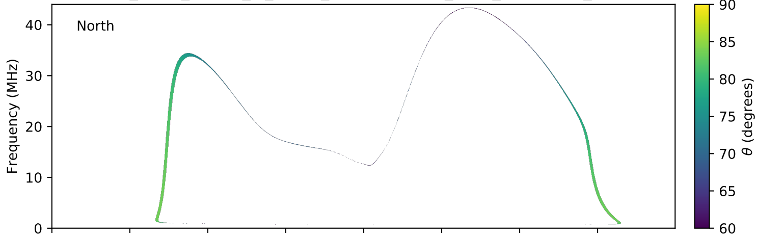
expres_earth_jupiter_io_jrm09_lossc-wid1deg_3kev_20060304_v01.cdf
