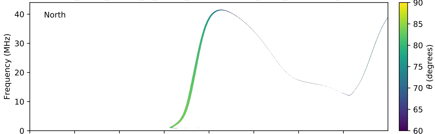
expres_earth_jupiter_io_jrm09_lossc-wid1deg_3kev_20060302_v01.cdf
