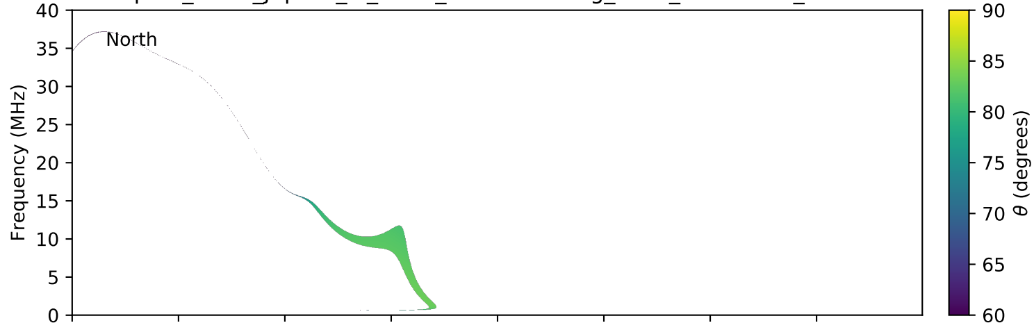
expres_earth_jupiter_io_isaac_lossc-wid1deg_3kev_20060331_v01.cdf
