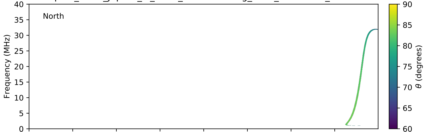
expres_earth_jupiter_io_isaac_lossc-wid1deg_3kev_20060328_v01.cdf
