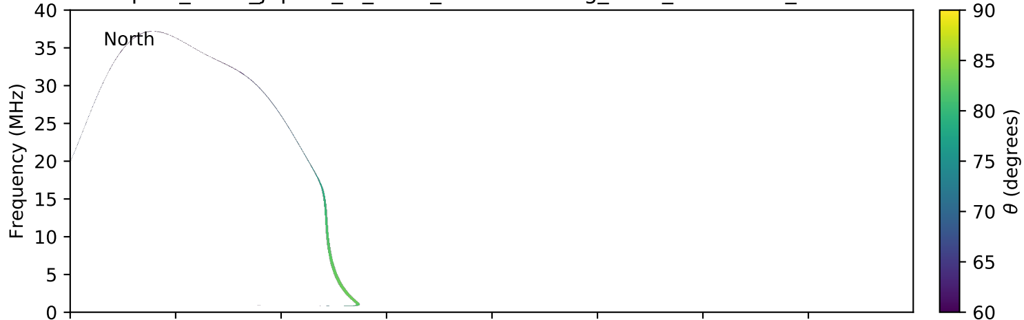
expres_earth_jupiter_io_isaac_lossc-wid1deg_3kev_20060324_v01.cdf
