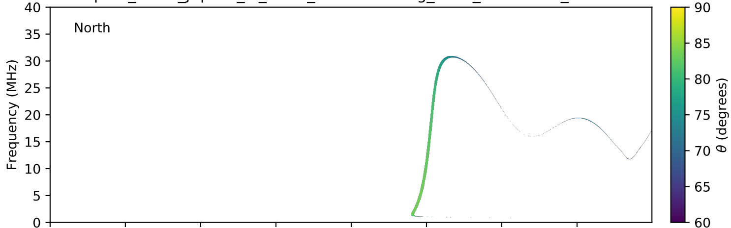
expres_earth_jupiter_io_isaac_lossc-wid1deg_3kev_20060323_v01.cdf
