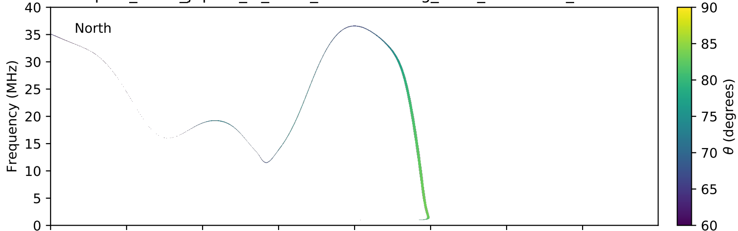
expres_earth_jupiter_io_isaac_lossc-wid1deg_3kev_20060322_v01.cdf
