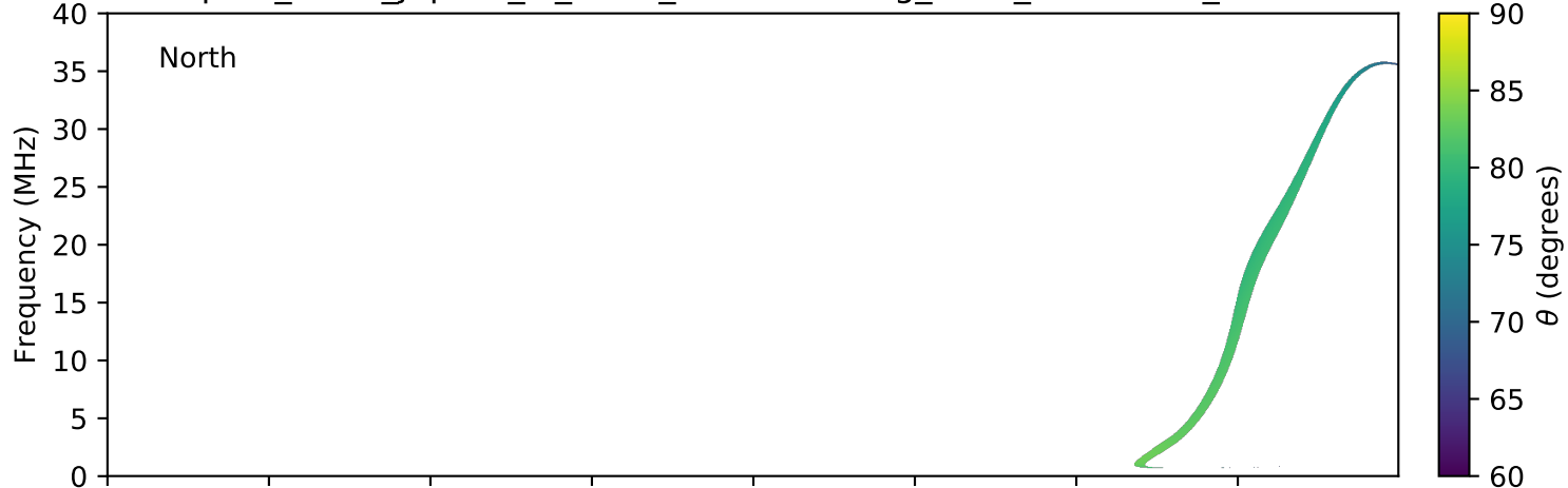
expres_earth_jupiter_io_isaac_lossc-wid1deg_3kev_20060321_v01.cdf
