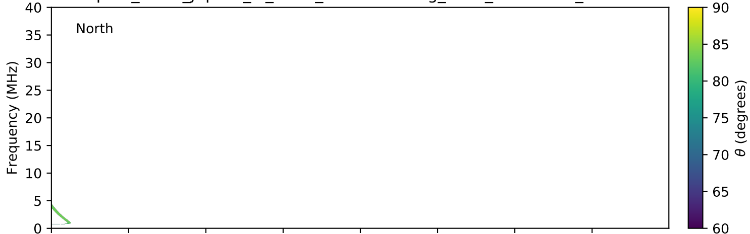
expres_earth_jupiter_io_isaac_lossc-wid1deg_3kev_20060319_v01.cdf
