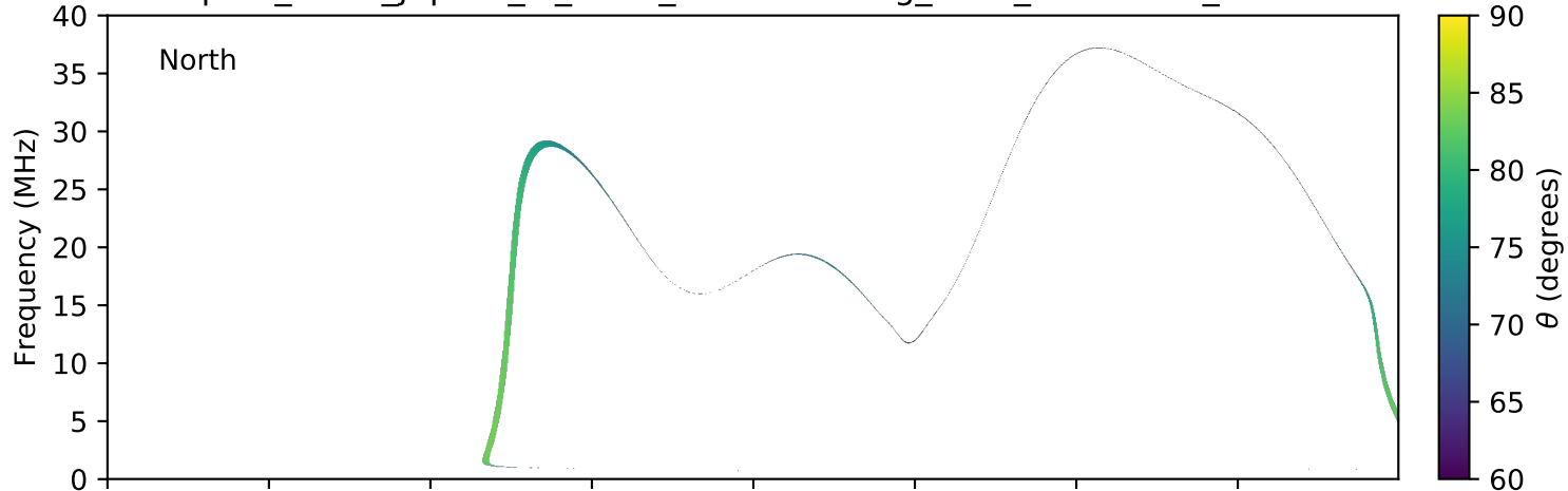
expres_earth_jupiter_io_isaac_lossc-wid1deg_3kev_20060318_v01.cdf
