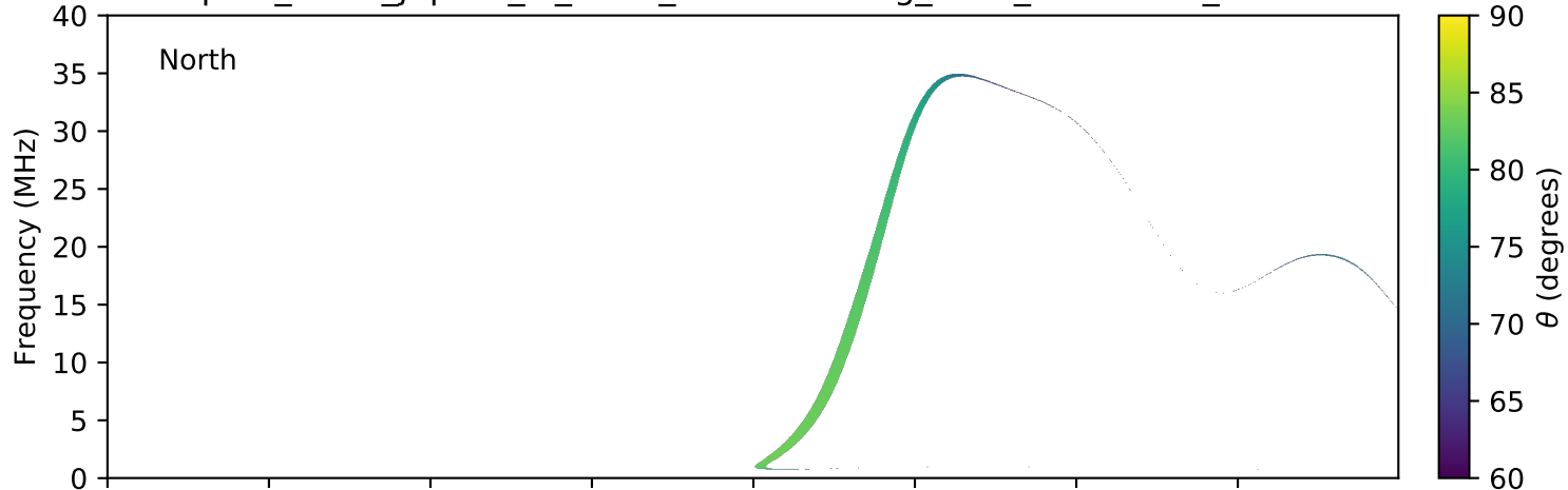
expres_earth_jupiter_io_isaac_lossc-wid1deg_3kev_20060316_v01.cdf
