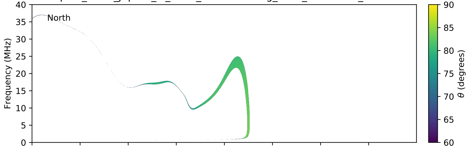
expres_earth_jupiter_io_isaac_lossc-wid1deg_3kev_20060315_v01.cdf
