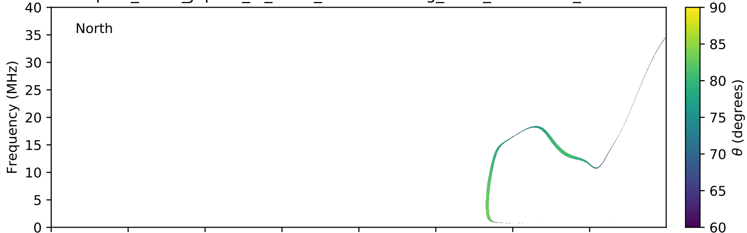
expres_earth_jupiter_io_isaac_lossc-wid1deg_3kev_20060314_v01.cdf
