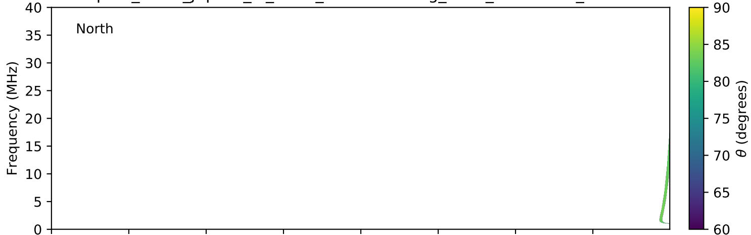
expres_earth_jupiter_io_isaac_lossc-wid1deg_3kev_20060312_v01.cdf
