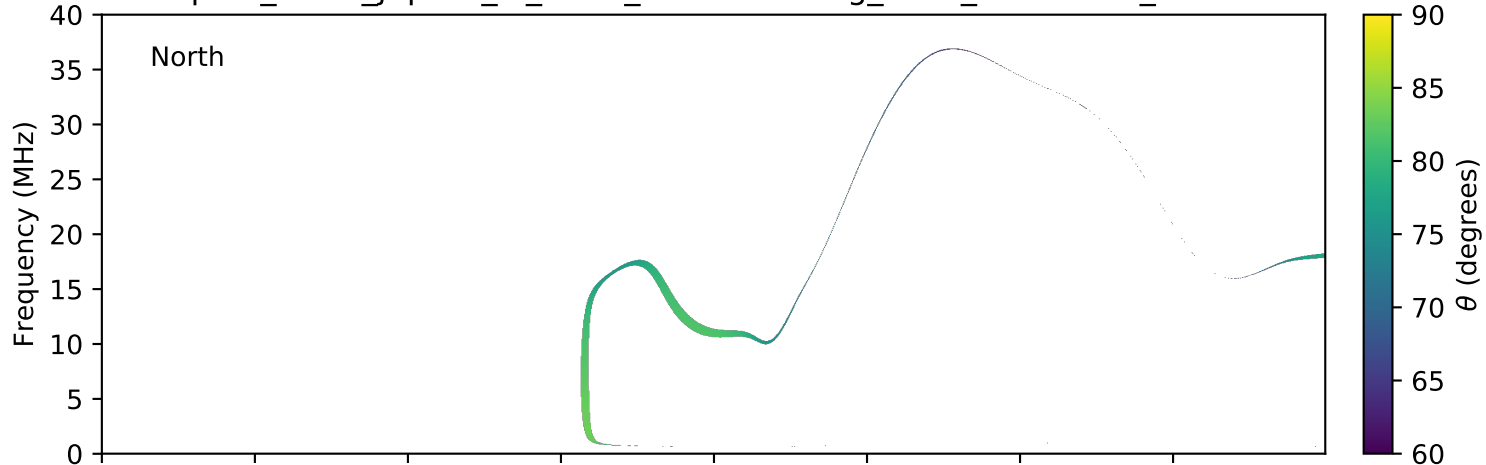
expres_earth_jupiter_io_isaac_lossc-wid1deg_3kev_20060309_v01.cdf
