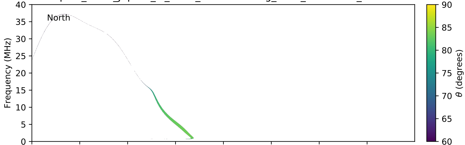
expres_earth_jupiter_io_isaac_lossc-wid1deg_3kev_20060308_v01.cdf
