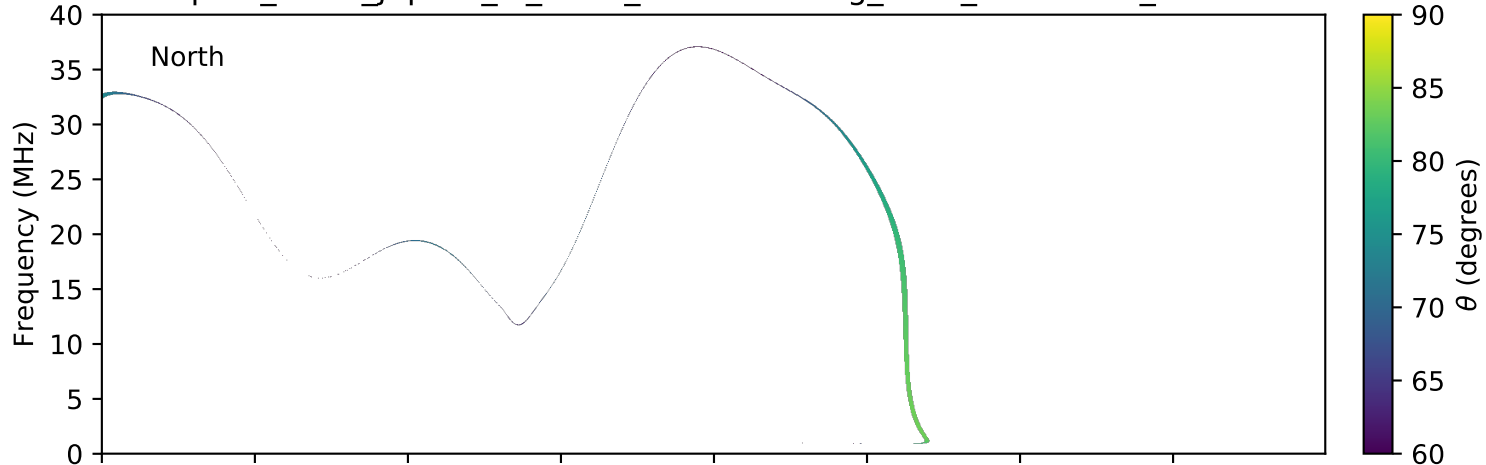
expres_earth_jupiter_io_isaac_lossc-wid1deg_3kev_20060306_v01.cdf
