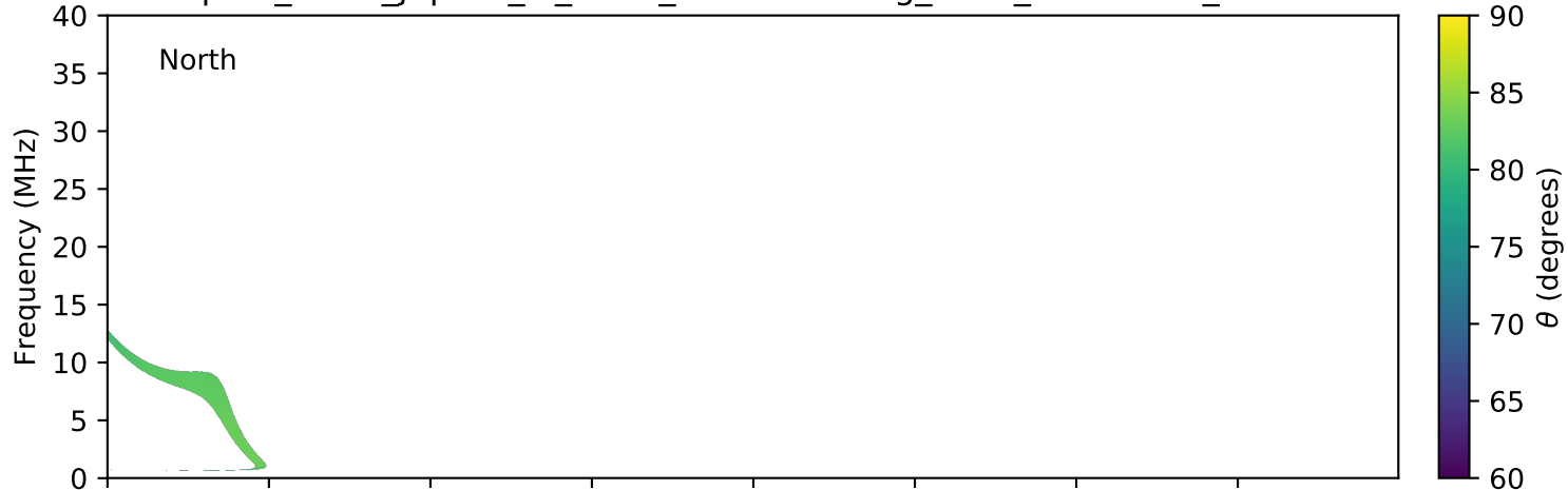
expres_earth_jupiter_io_isaac_lossc-wid1deg_3kev_20060303_v01.cdf
