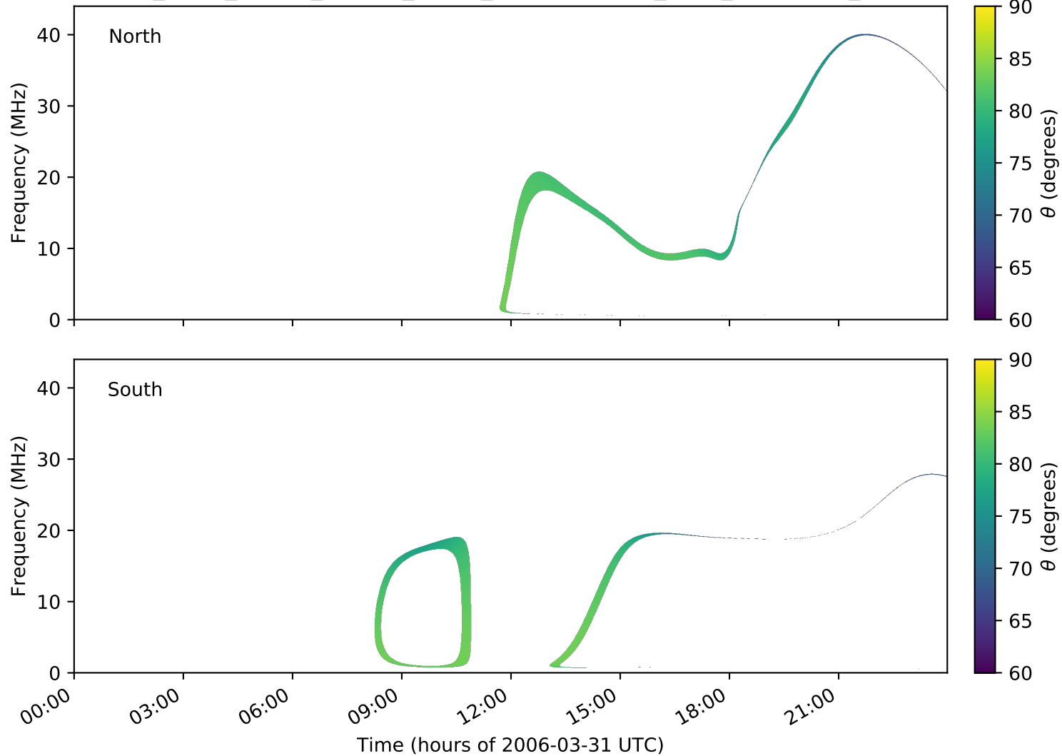
expres_earth_jupiter_europa_jrm09_lossc-wid1deg_3kev_20060331_v01.cdf
