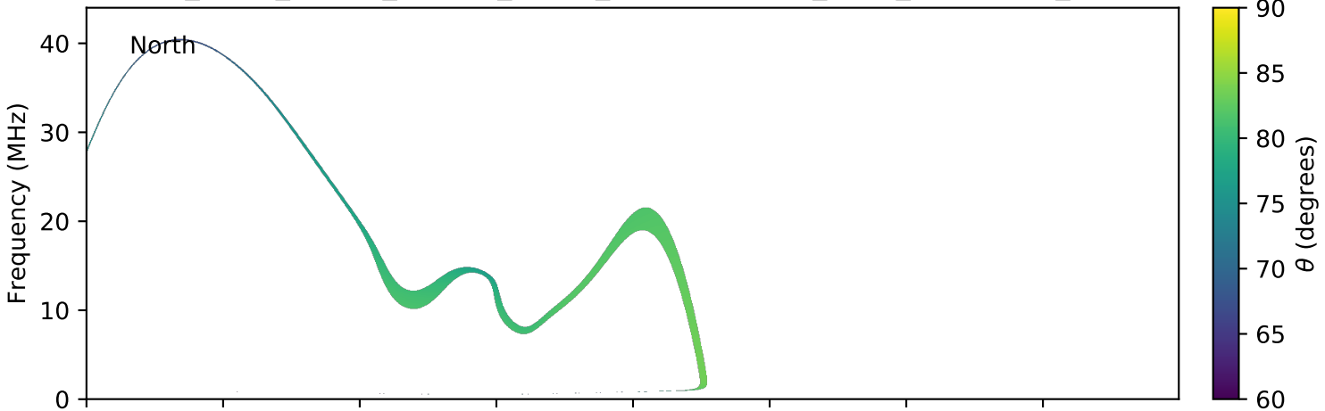
expres_earth_jupiter_europa_jrm09_lossc-wid1deg_3kev_20060329_v01.cdf
