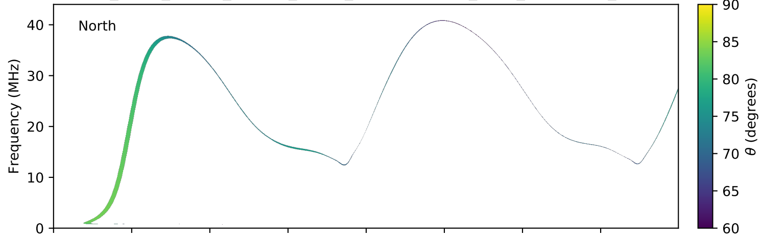
expres_earth_jupiter_europa_jrm09_lossc-wid1deg_3kev_20060328_v01.cdf
