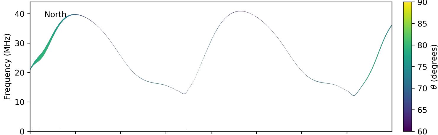
expres_earth_jupiter_europa_jrm09_lossc-wid1deg_3kev_20060314_v01.cdf
