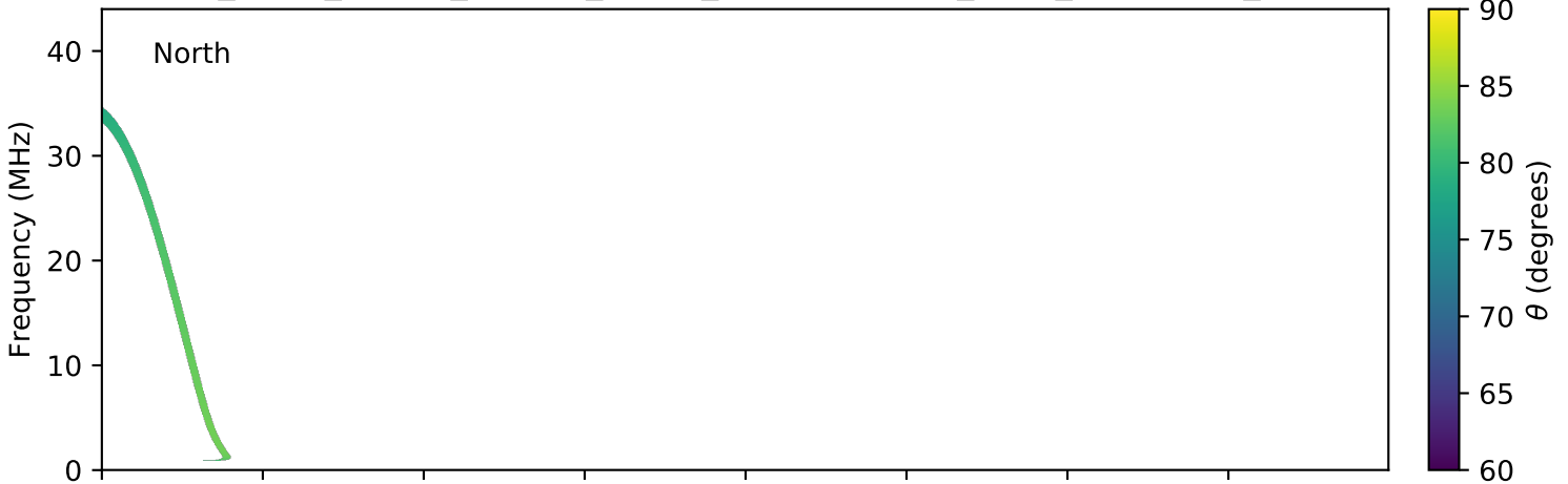
expres_earth_jupiter_europa_jrm09_lossc-wid1deg_3kev_20060301_v01.cdf
