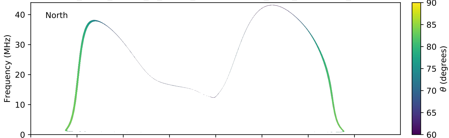
expres_earth_jupiter_io_jrm09_lossc-wid1deg_3kev_20060225_v01.cdf
