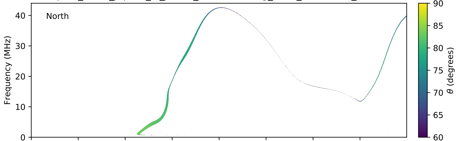
expres_earth_jupiter_io_jrm09_lossc-wid1deg_3kev_20060223_v01.cdf
