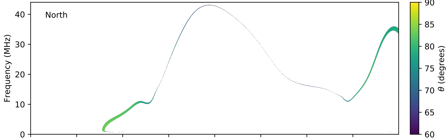
expres_earth_jupiter_io_jrm09_lossc-wid1deg_3kev_20060216_v01.cdf
